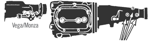
Vega/Monza SAGINAW, G.M. (441) 7-bolt side cover Holes may not be tapped
